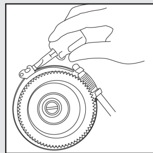
Loosen adjustor clamp
